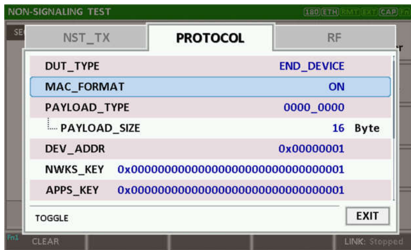
Fig 3.32 PROTOCOL Parameters 1/2 for Signal Generator
