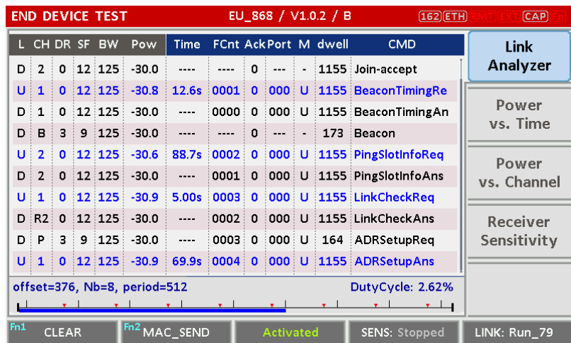
Fig 3.17 MAC command transmission through PING slot
