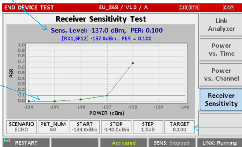
Fig 2.14 Receiver Sensitivity Screen
