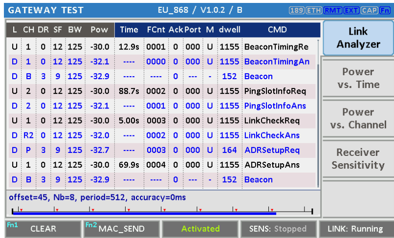
Fig 3.30 Example of communication with Class B Gateway
