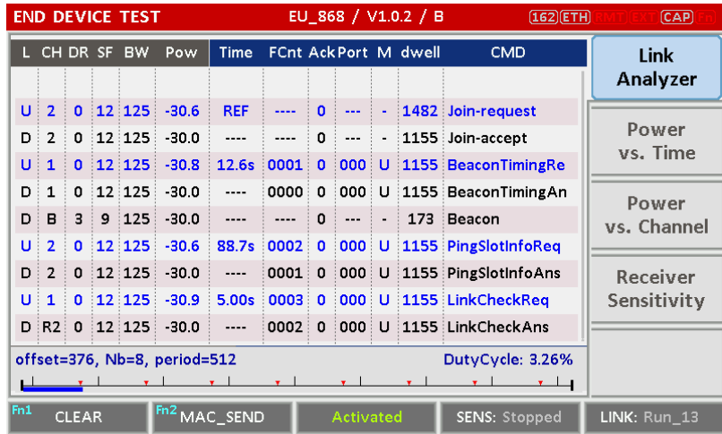
Fig 3.15 Example of communication with Class B End Device
